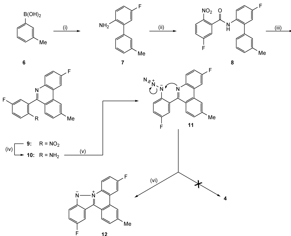
Scheme 1 Attempted synthesis of quino[4,3,2- k ]acridine 4 from a 2-arylphenanthridine precursor (Route A). Reagents and conditions: (i) 2-bromo-4-fluoroaniline, tetrakis triphenylphosphine palladium (5 mol%), Na 2 CO 3 , DME–EtOH–H 2 O under nitrogen, reflux; (ii) 2-nitro-5-fluorobenzoic acid, DCC in CHCl 3 , 25 °C; (iii) POCl 3 , 90 °C; (iv) tin(II) chloride dihydrate, EtOH, reflux, then NaOH; (v) NaNO 2 , 1 M H 2 SO 4 , 5 °C, then NaN 3 ; (vi) 214 °C in 1,2,4-trichlorobenzene.
