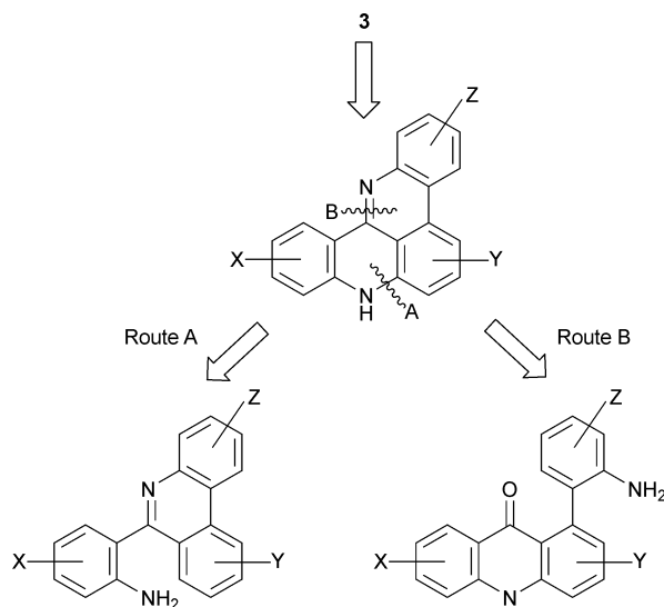
Fig. 2 Synthetic strategies to trisubstituted quino[4,3,2- k ]acridines.
