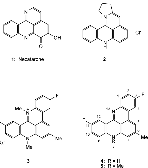
Fig. 1 Structures of bioactive polycyclic acridines and numbering of the quino[4,3,2- kl ]acridine ring system.
