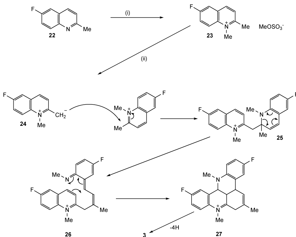
Scheme 3 Synthesis of quino[4,3,2- k ]acridine 3 from 6-fluoro-2-methylquinoline (Route C). Reagents and conditions: (i) Me 2 SO 4 at 100 °C; (ii) NEt 3 in nitrobenzene, 120 °C, 24 h.
