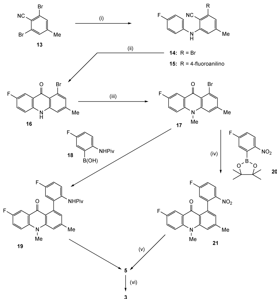
Scheme 2 Synthesis of quino[4,3,2- k ]acridine 3 from a 1-arylacridin-9(10 H )-one precursor (Route B). Reagents and conditions: (i) 4-fluoroaniline, Pd(OAc) 2 , BINAP, Cs 2 CO 3 , toluene, 100 °C; (ii) 80% H 2 SO 4 , 100 °C; (iii) NaH in DMF, Me 2 SO 4 ; (iv) 17 and 20 in dioxan, PdCl 2 (dppf) (10 mol%), Na 2 CO 3 , 80 °C; (v) tin(II) chloride dihydrate, EtOH, reflux; (vi) Me 2 SO 4 in MeNO 2 , reflux.
